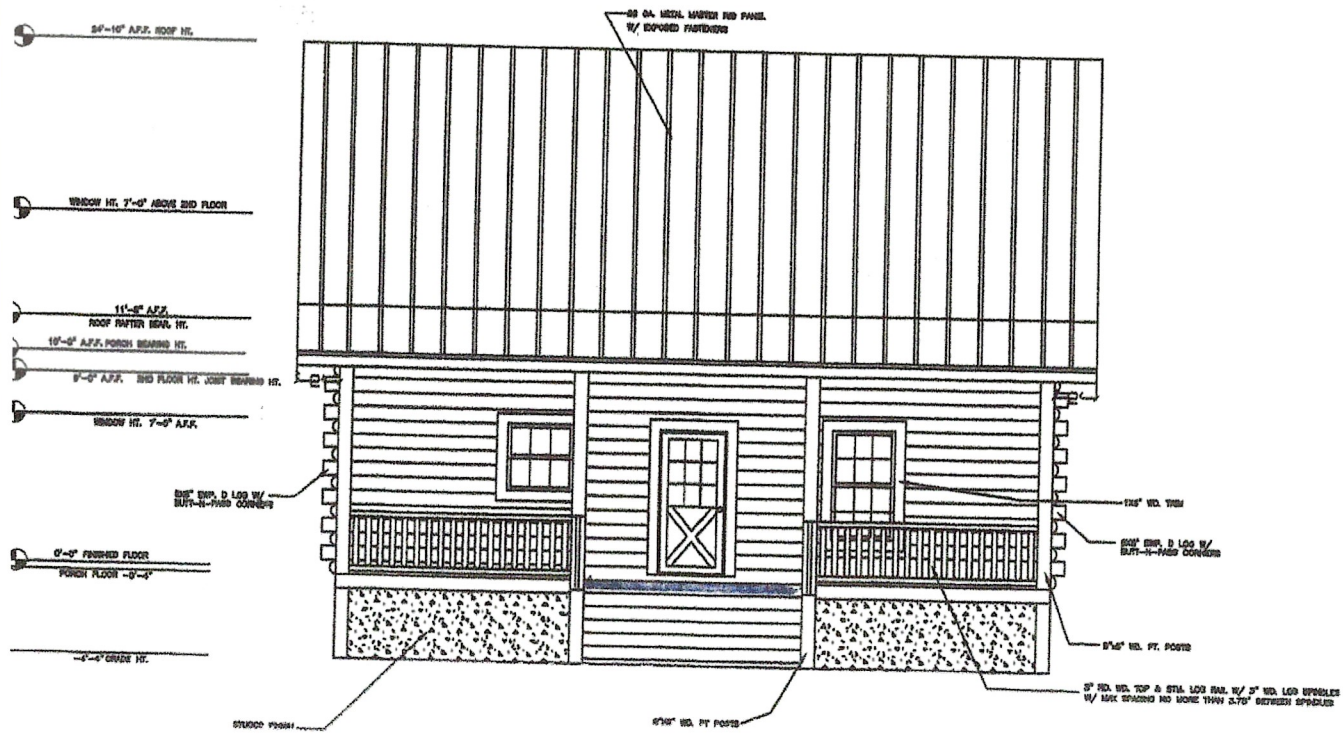
FRONT ELEVATION
